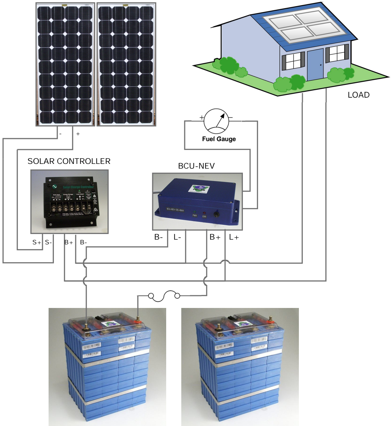
EV POWER PAK LFP BATTERY 12V/24V 40-400Ah
